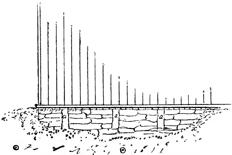
Fig. 110—Wall with Openings for the Roots
